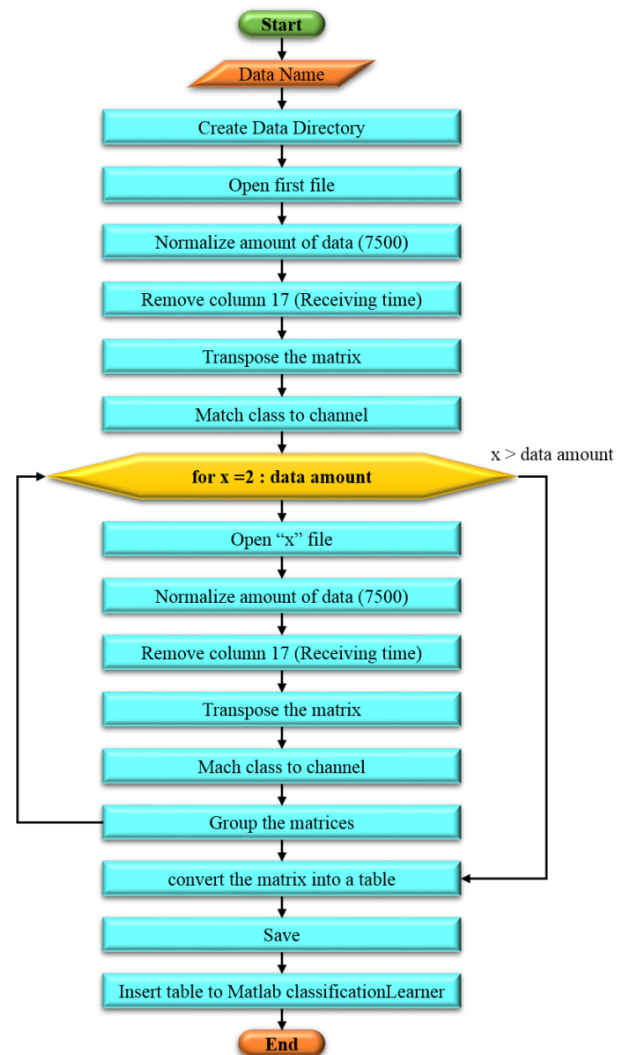
Fig. 4. Flow Chart for Grouping the Data.
